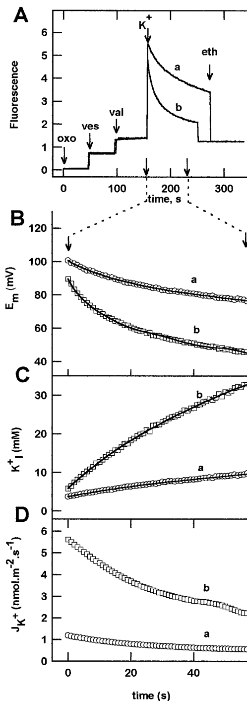
FIGURE 7 Determination of net ion fluxes from depolarization kinetics of \text{K}^+ -valinomycin diffusion potentials. (A) Fluorescence records at \text{pH } 6.5 after successive additions of oxonol VI, reconstituted PM vesicles, valinomycin, and \text{K}_2\text{SO}_4 (trace a), or \text{K}_2\text{SO}_4 plus \text{KNO}_3 (trace b), to make the final concentration of \text{K}^+ and \text{NO}_3^- equal to 200 \text{ mM} and 15 \text{ mM} , respectively. The \text{Li}^+ -ionophore eth was added at the end of the assay to clamp E_m to zero, both external and internal media containing \text{Li}^+ . (B) E_m ( E_{\text{probe3}} , Eq. 7) was calculated from the four fluorescence intensities indicated in Fig. 1. (C) Internal \text{K}^+ concentration ( \text{K}_i^+ ) at equilibrium with E_m was calculated (Eq. 8) and fitted using a polynomial regression algorithm (solid line). (D) Net \text{K}^+ fluxes ( J_K ) in the presence and in the absence of \text{NO}_3^- were calculated from the derivatives of the polynomial fits (Eq. 9), and the net \text{NO}_3^- flux ( J_N ) was determined as the \text{NO}_3^- -dependent augmentation of J_K (see text).
