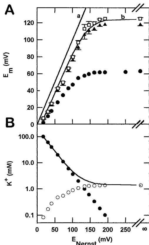
FIGURE 6 \text{K}^+ -valinomycin diffusion gradients across reconstituted PM vesicles or control liposomes: comparison of experimental potentials given by the oxonol VI probe and expected \text{K}^+ Nernst potentials. (A) The diffusion potential in response to increasing \text{K}^+ -valinomycin gradients was experimentally determined ( E_m ) from the oxonol VI fluorescence and plotted versus the Nernst potential expected from the initially imposed \text{K}^+ -valinomycin gradient ( E_{\text{Nernst}} = (RT/F)\ln(K_o^+/K_i^+) ). Three experimental E_m estimates were calculated (Eq. 5) from the fluorescence ratio R_{t_i} = \Delta F_i/F_o , measured as described in Fig. 1 and shown in Fig. 3: E_{\text{probe1}} (●) calculated from R_{t_i} without any correction; E_{\text{probe2}} (▲) from R_{t_i} corrected for dye depletion (Eq. 6); E_{\text{probe3}} (□) from R_{t_i} corrected for both dye depletion and dye saturation of the internal vesicle leaflet (Eq. 7). Reference E_{\text{Nernst}} values are also plotted (curve a) to facilitate comparison. Curve b corresponds to the theoretical potential expected from capacitive effects on diffusion potential across membrane vesicles (Eq. 4, with C_m = 1 \mu\text{F cm}^{-2} , r = 28 \text{ nm} ; see Materials and Methods and Table 2); the \text{K}^+ concentrations in the lumen ( \text{K}_i^+ ) introduced in this calculation were those at equilibrium with the negative-inside Donnan potential expected before the imposition of the \text{K}^+ gradient (Eq. 8). (B) Comparison of the \text{K}^+ concentration initially present in the lumen of the vesicles ( \text{K}_i^+ , ●) and the equivalent \text{K}^+ concentration to be transferred in the lumen to charge the membrane capacitor according to Eq. 2 ( \text{K}_{\text{eq}}^+ , ○); the solid line indicates the total internal concentration of \text{K}^+ ( \text{K}_t^+ = \text{K}_i^+ + \text{K}_{\text{eq}}^+ ) theoretically expected at initial equilibrium E_m ; the increasing discrepancy between E_{\text{probe3}} and E_{\text{Nernst}} is observed (see A) when \text{K}_{\text{eq}}^+ becomes significant compared to \text{K}_i^+ .
